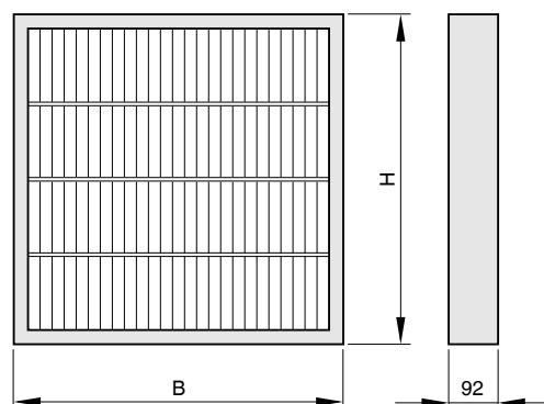
Dimensional drawing of KM, 92 mm
