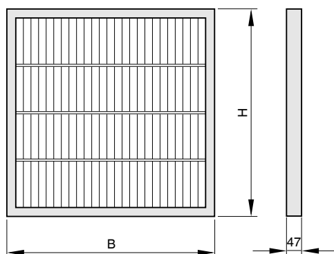
Dimensional drawing of KM, 47 mm
